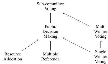
Figure 1: Relations between settings. An arrow from (A) to (B) denotes that setting (A) is a restriction of setting (B).
